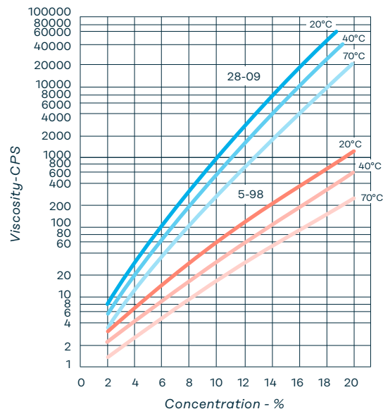
Figure 2: Viscosity Concentration Relationship for Aqueous Solutions of Kuraray Poval™ at Various Temperatures
